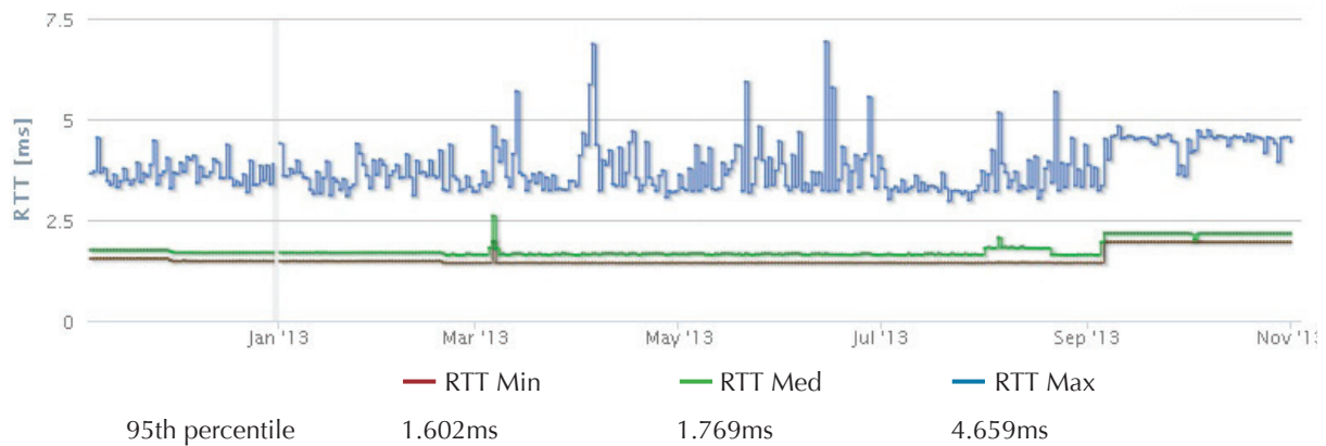
Abb.2 i-root-annual IPv6
